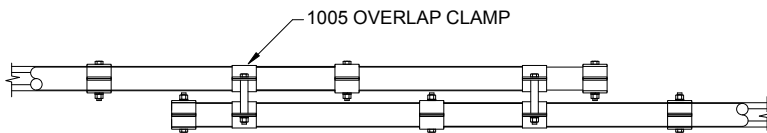
OVERLAP
