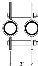
SECTION AT OVERLAP
