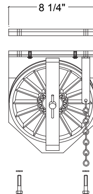
1024 SINGLE END PULLEY
