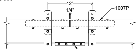
SPLICE
