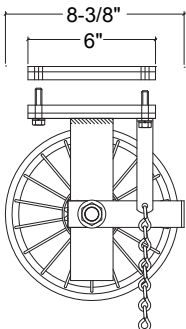
1023 DOUBLE END PULLEY
