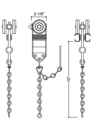
1018 SINGLE CARRIER
