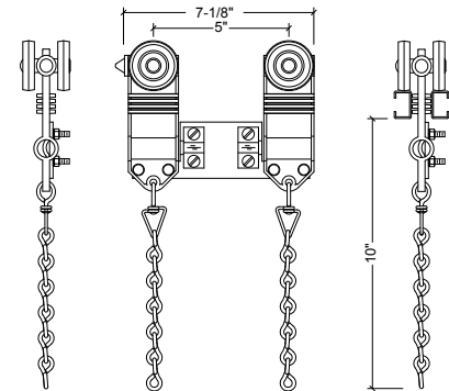
1019 MASTER CARRIER
